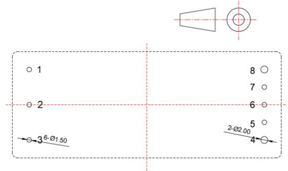
Recommended holes for PCB layout
